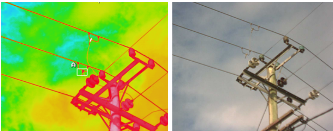
Figure 3: A Live Line Clamp through a thermal imaging camera and a normal camera
