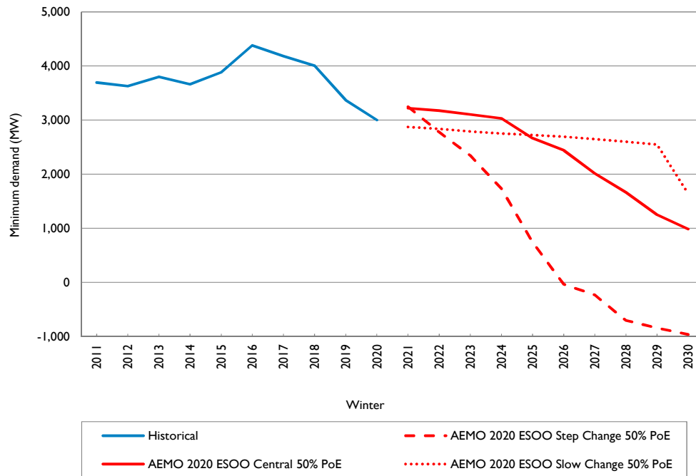
Figure 2.11 Historical and forecast winter transmission delivered minimum demand
