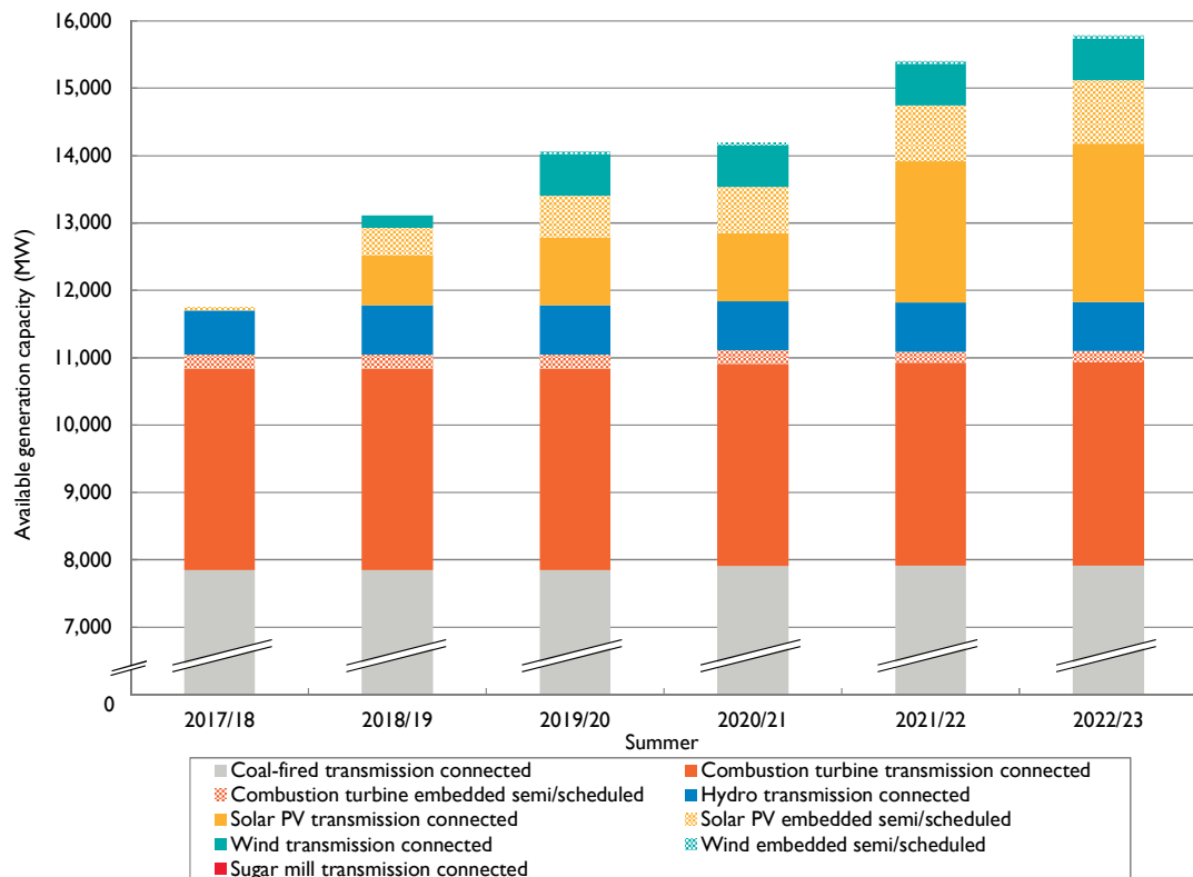
Figure 6.1 Summer available generation capacity by energy source
