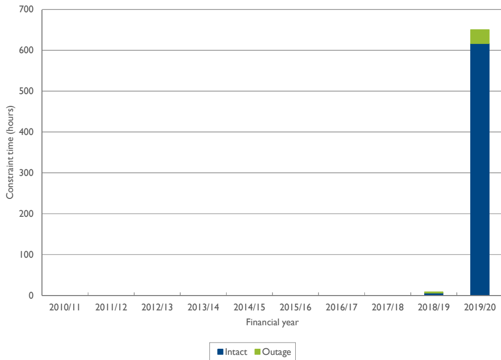
Figure 6.14 Historical NQ system strength constraint times
