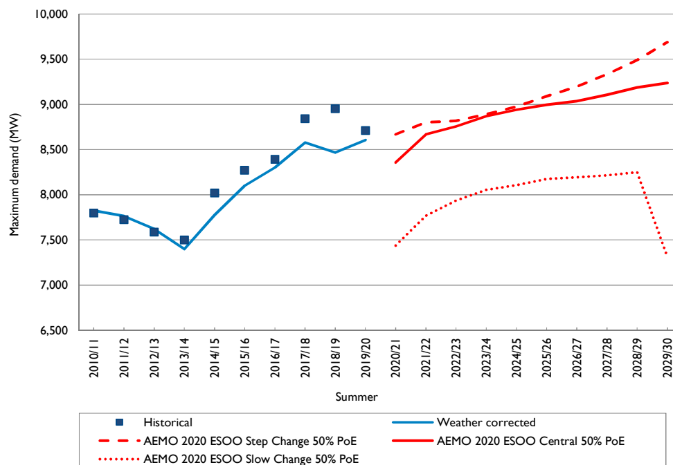
Figure 2.8 Historical and forecast transmission delivered summer maximum demand
