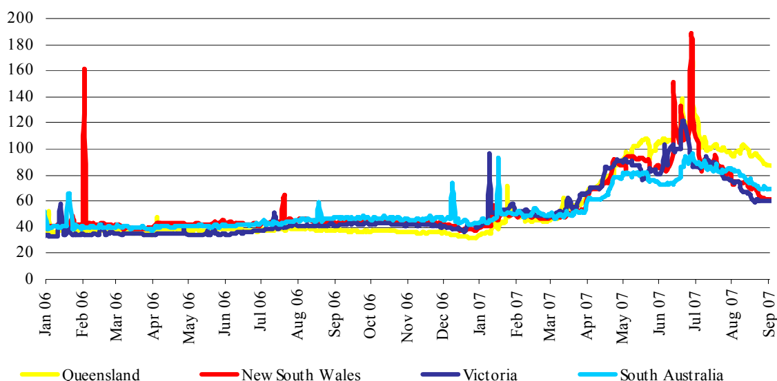
Figure 10: d-cyphaTrade WEPI
