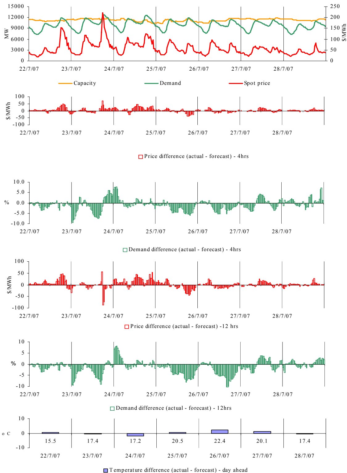
Figures 33-38 New South Wales actual spot price, demand and forecast differences
