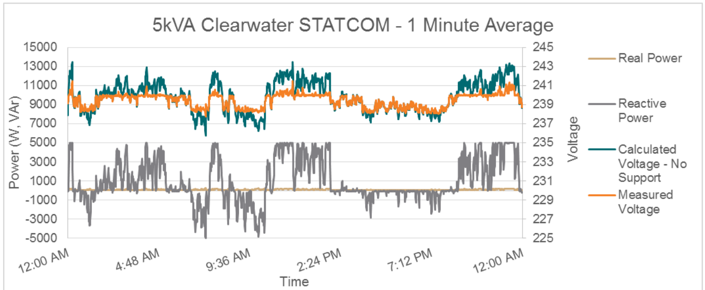
Figure 10 Clearwater 5kVA Inverter Results as at March 2015
