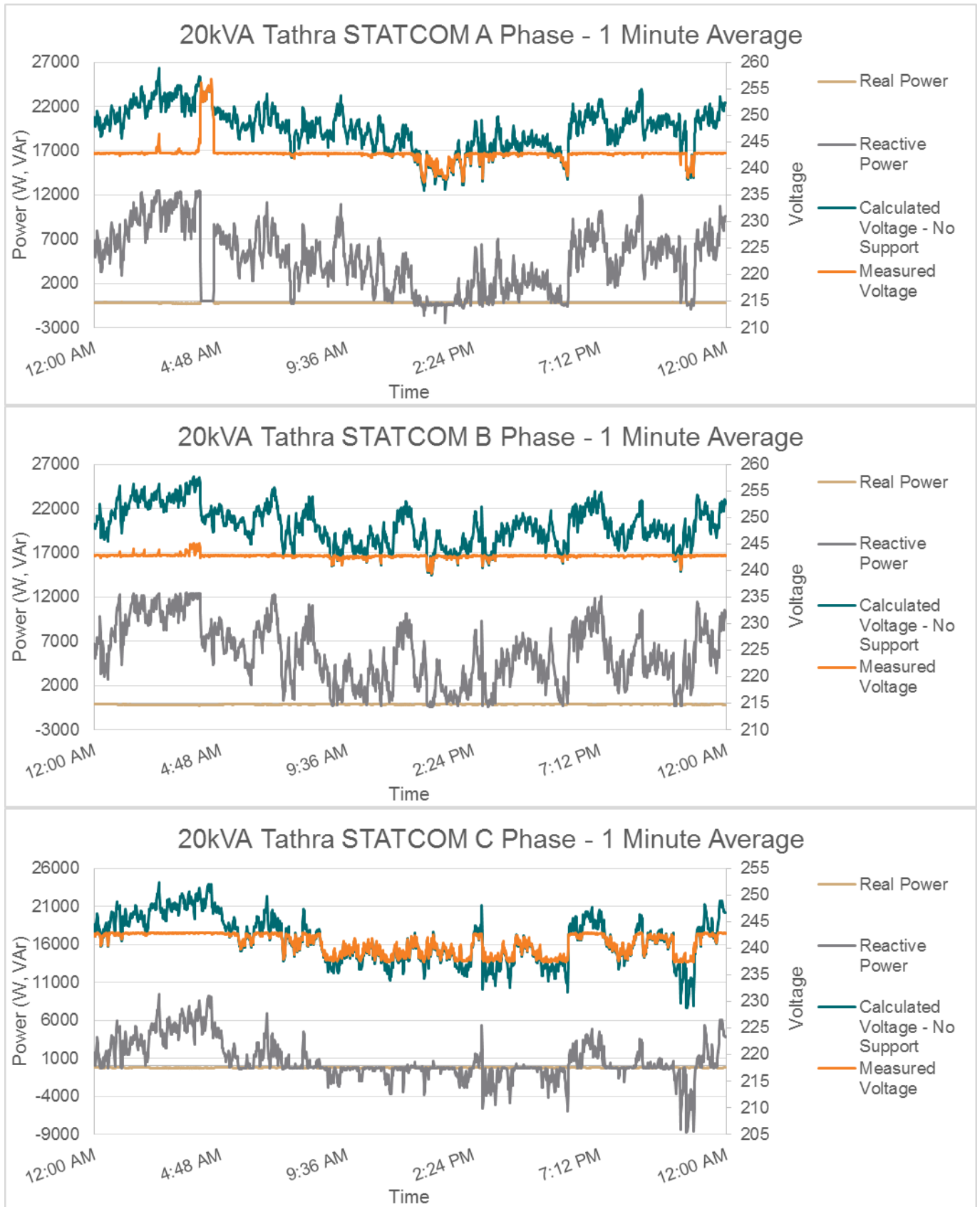
Figure 5 Tathra STATCOM with an over-temperature trip at 4:03 AM
