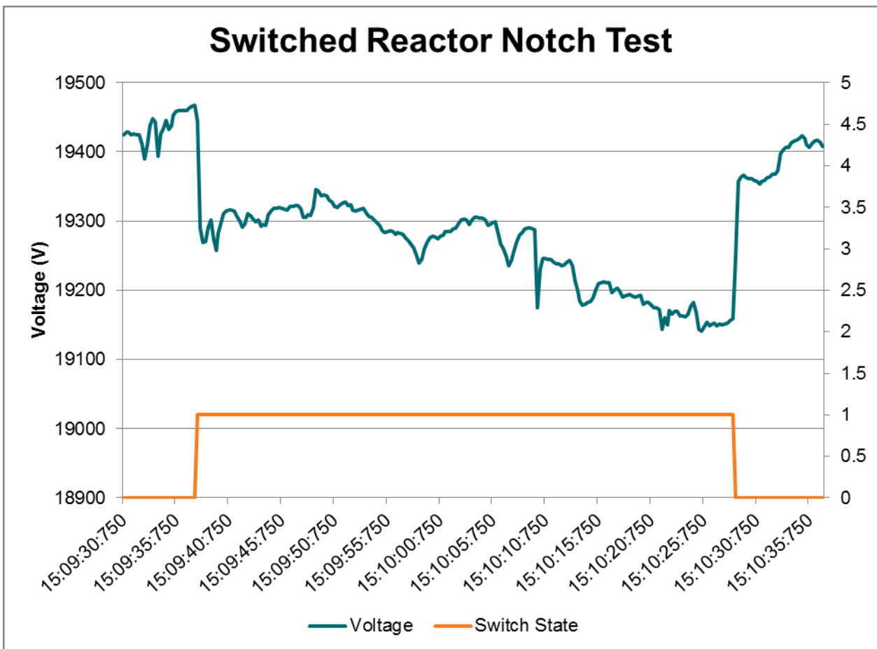
Figure 16: Switched Reactor Notch Test
