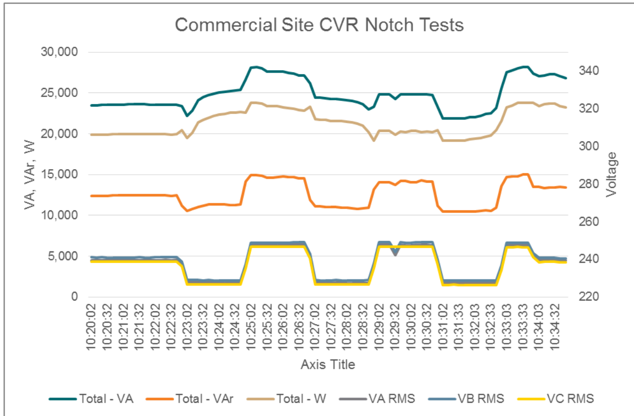
Figure 14 Notch testing to calculate CVRf of a commercial load
