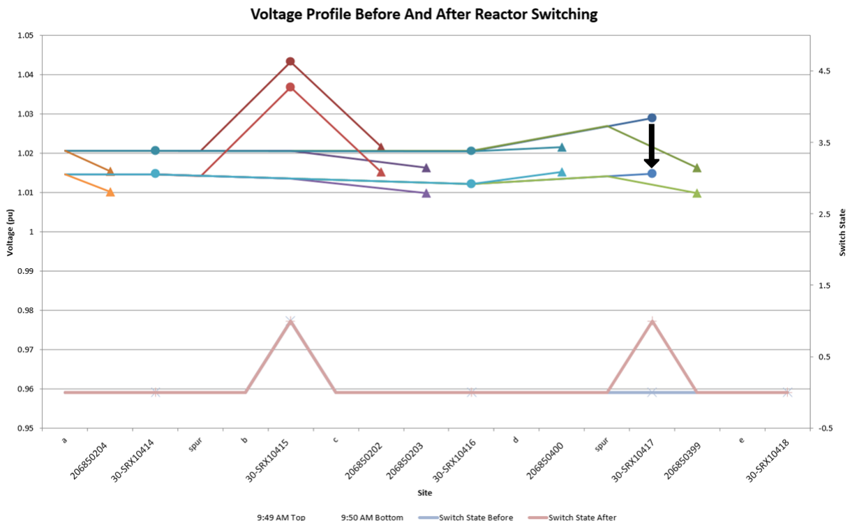
Figure 18 Nyngan network - 30-SRX10417 switch event
