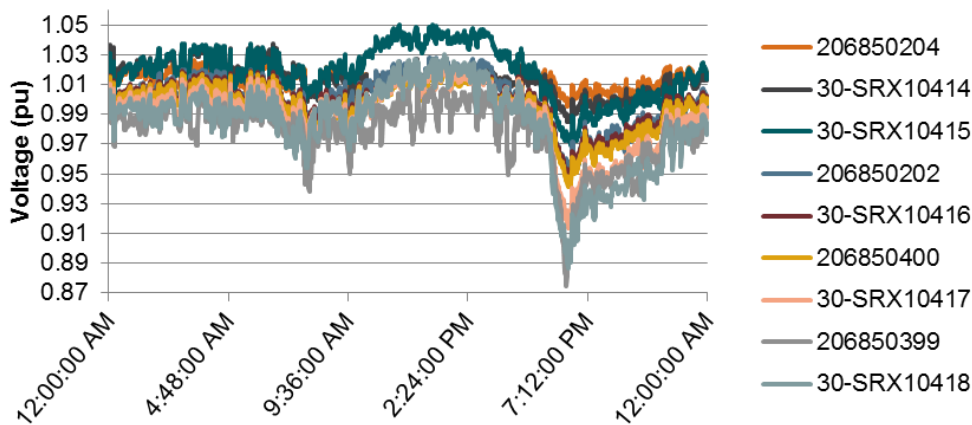
Figure 17 Nyngan network Voltage profile before Switched Reactors were placed in service
