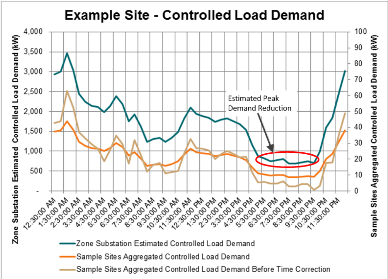
Figure 19: Sample Site Estimated Peak Demand Reduction
