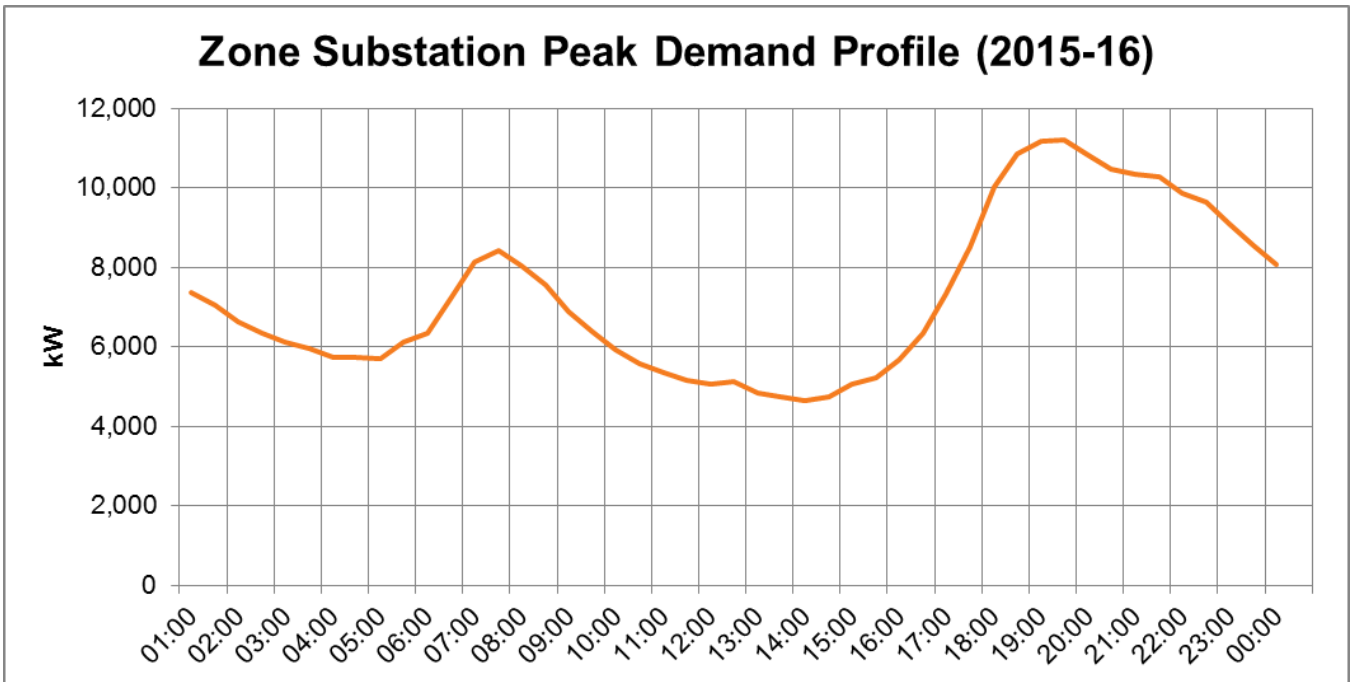
Figure 20: Sample Site Peak Demand Profile
