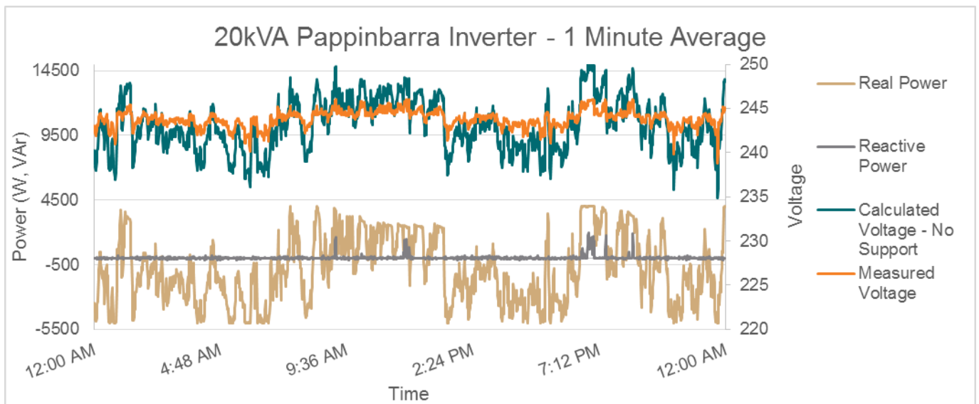
Figure 7 Pappinbarra Results as at July 2014
