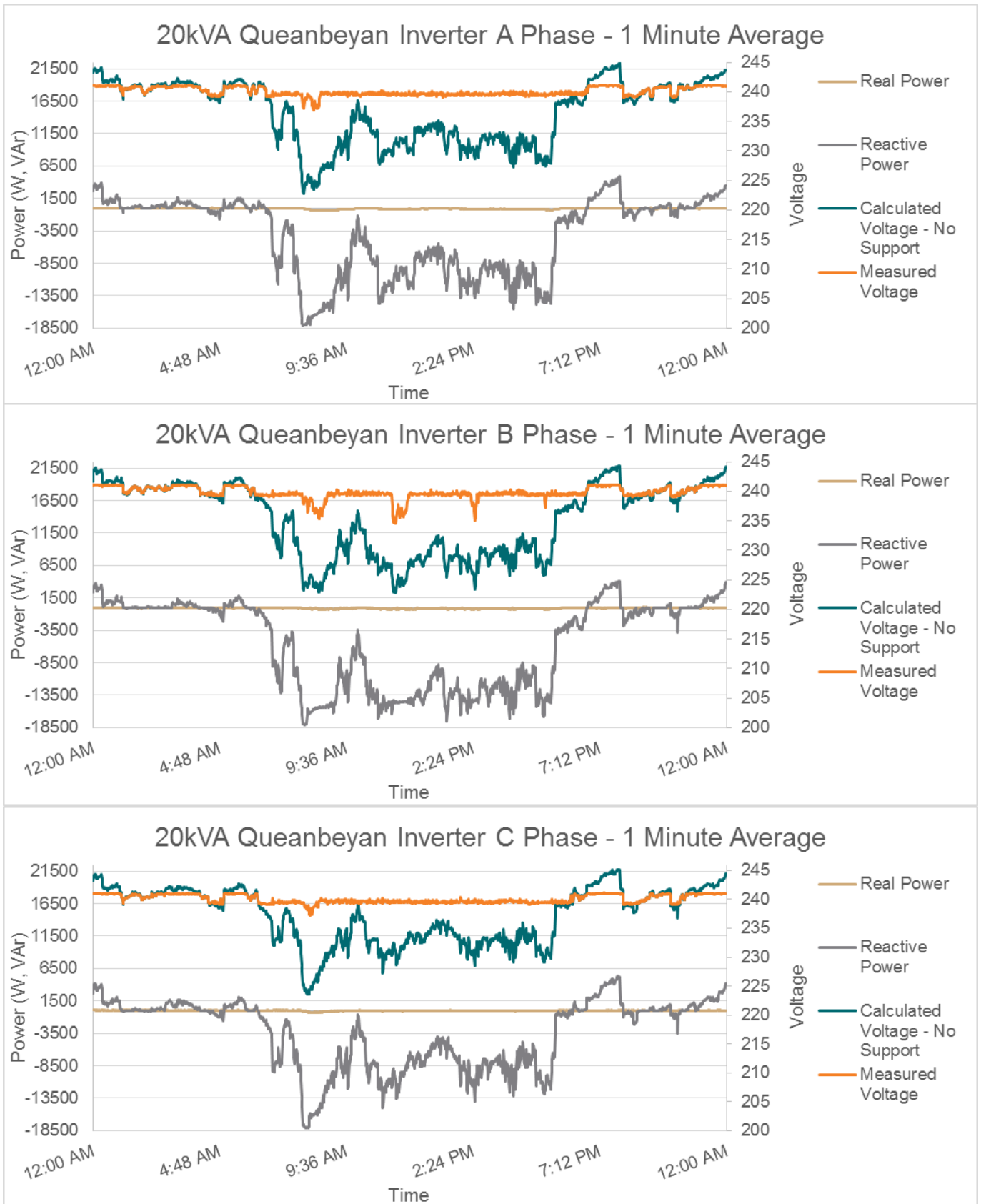
Figure 2 Queanbeyan Results as at October 2013
