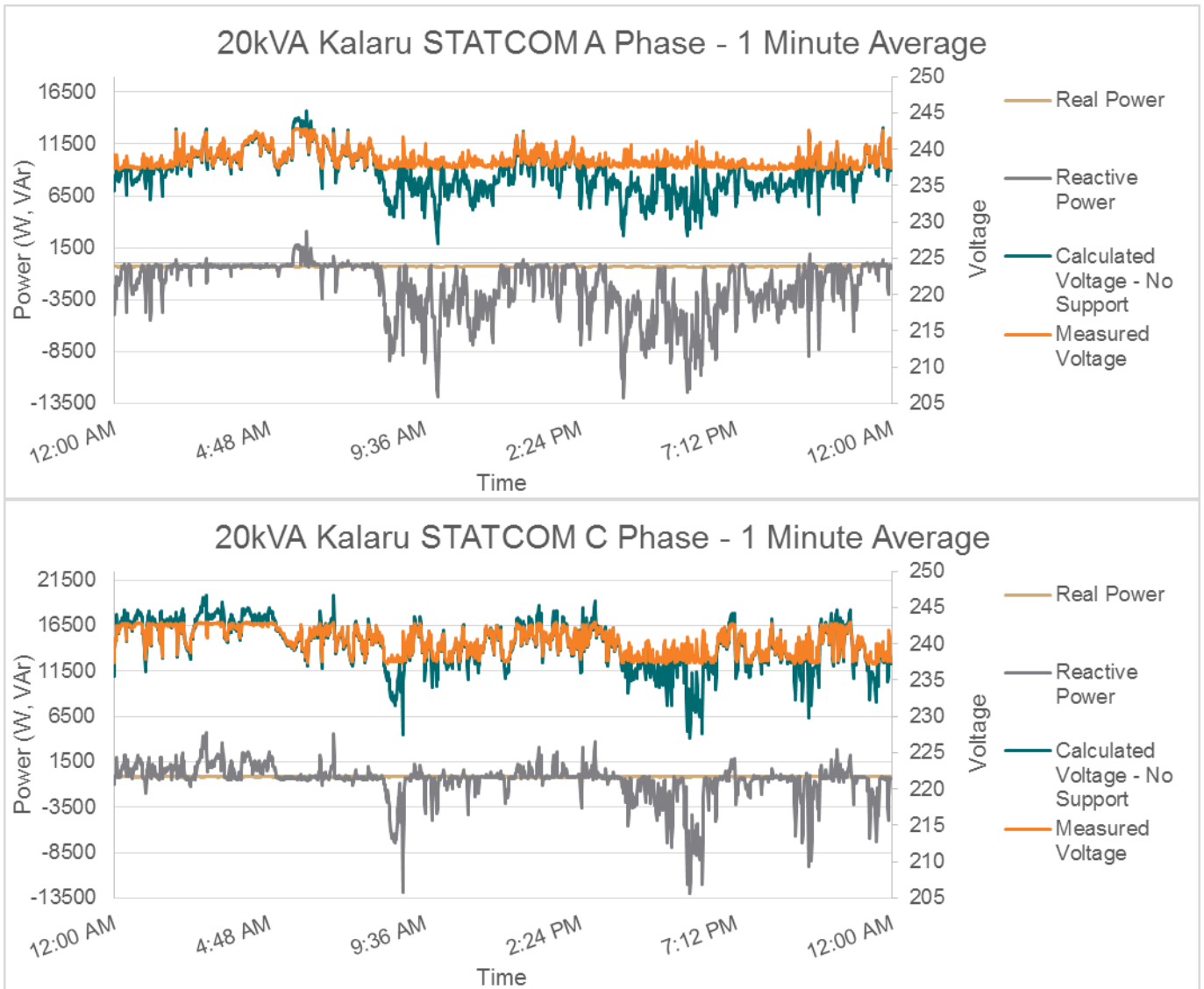
Figure 4 Kalaru results as at July 2012, B phase had a communications issue
