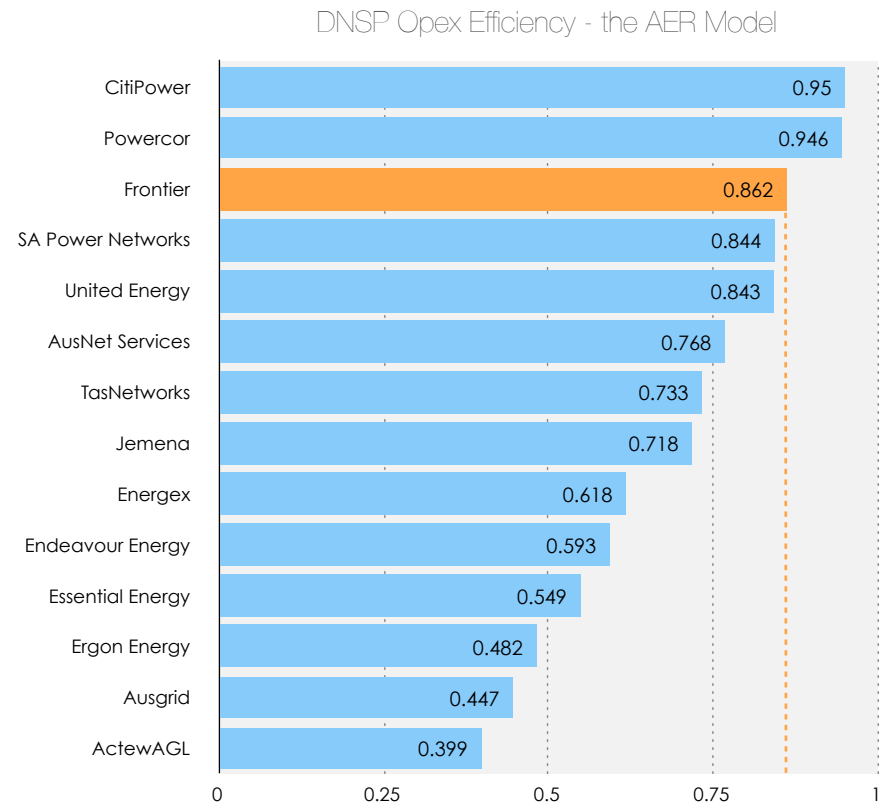
Figure 2: Opex efficiency scores from the AER model
