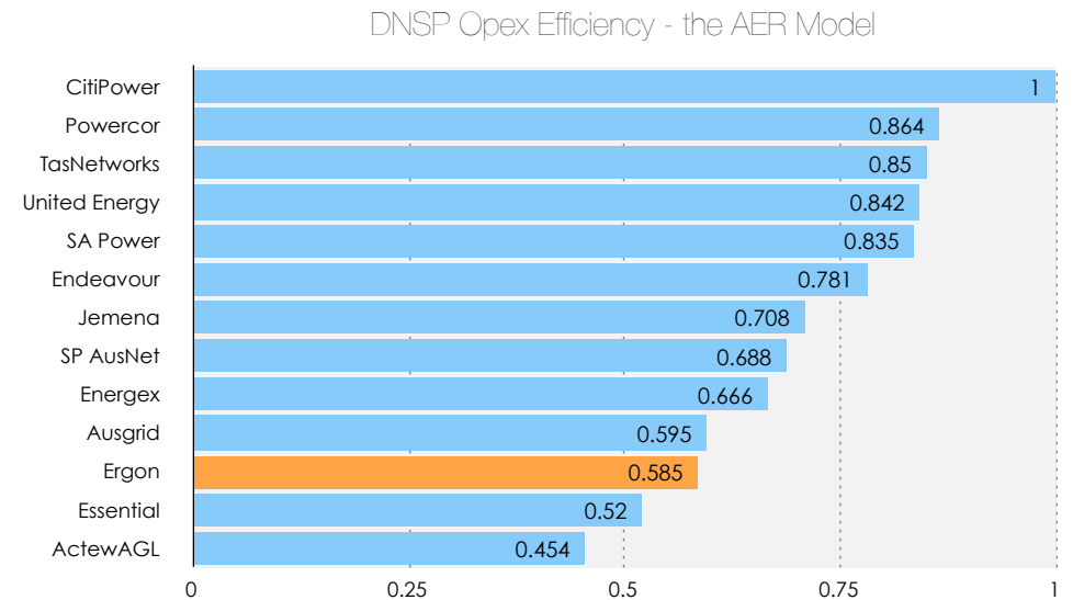
Figure 10: Opex PFP scores - AER and Huegin adjusted
