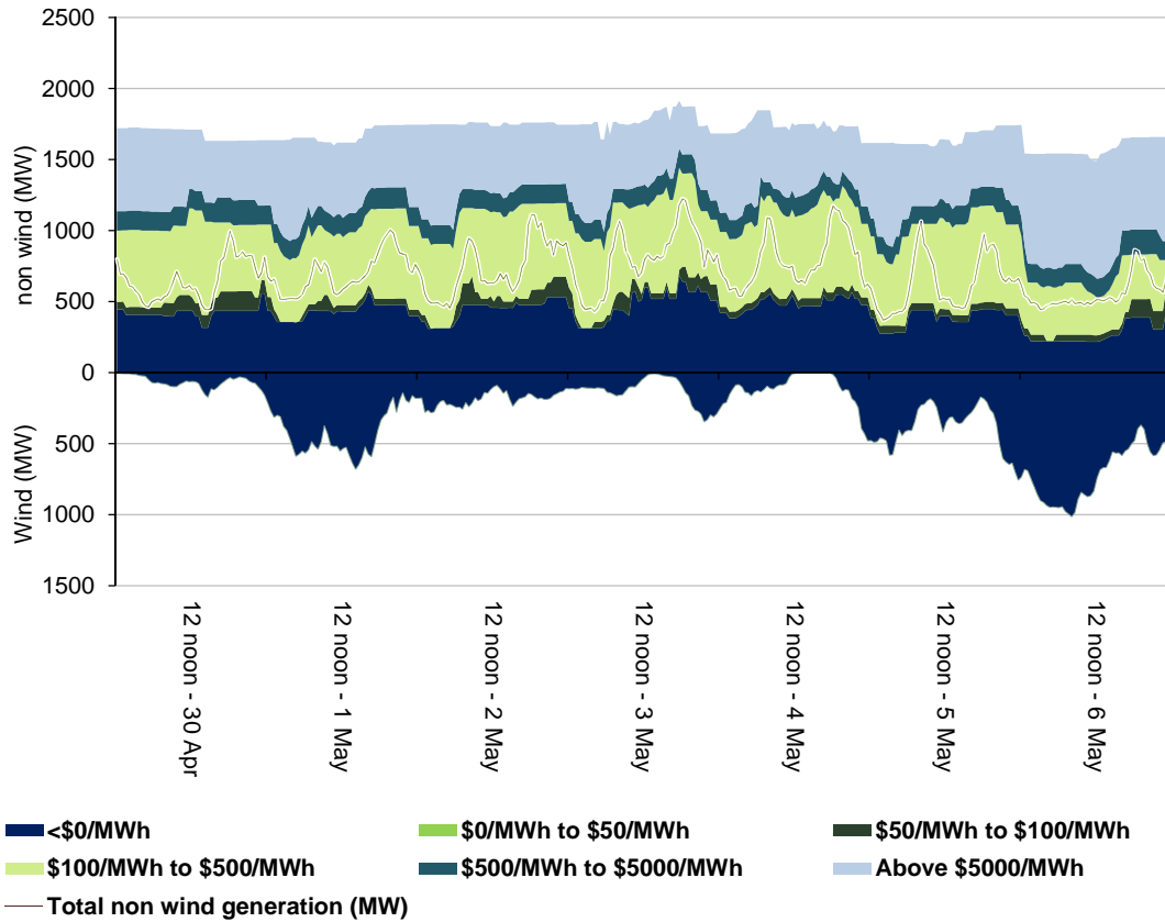
Figure 7: Tasmania generation and bidding patterns
