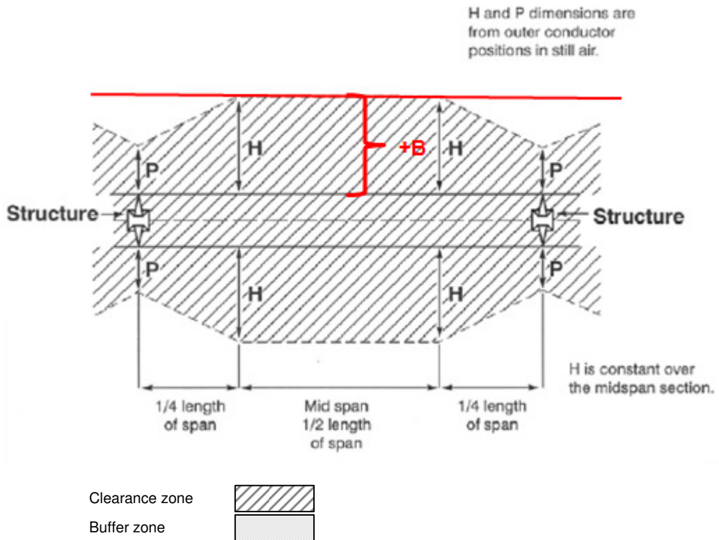
Figure 2-5: Overhead View Vegetation Corridor Clearances
