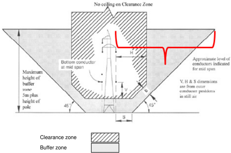
Figure 2-4: Vegetation Clearance Corridor – Bushfire Risk Area 132kV to 275kV
