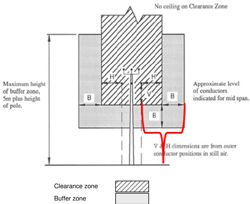
Figure 2-1: Vegetation Clearance Corridor – Non Bushfire Risk Area 33kV to 66kV
