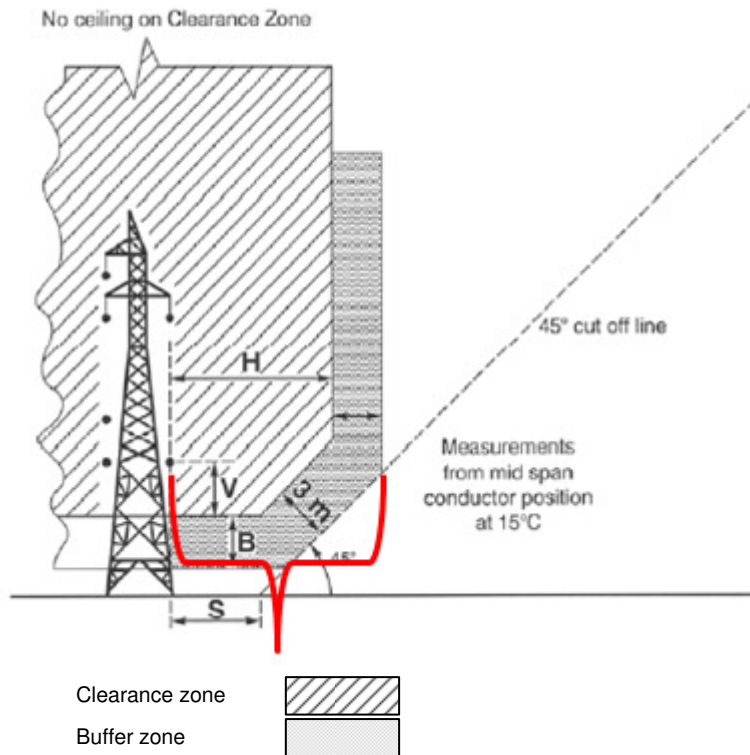
Figure 2-2: Vegetation Clearance Corridor - Non Bushfire Risk Area 132kV to 275kV
