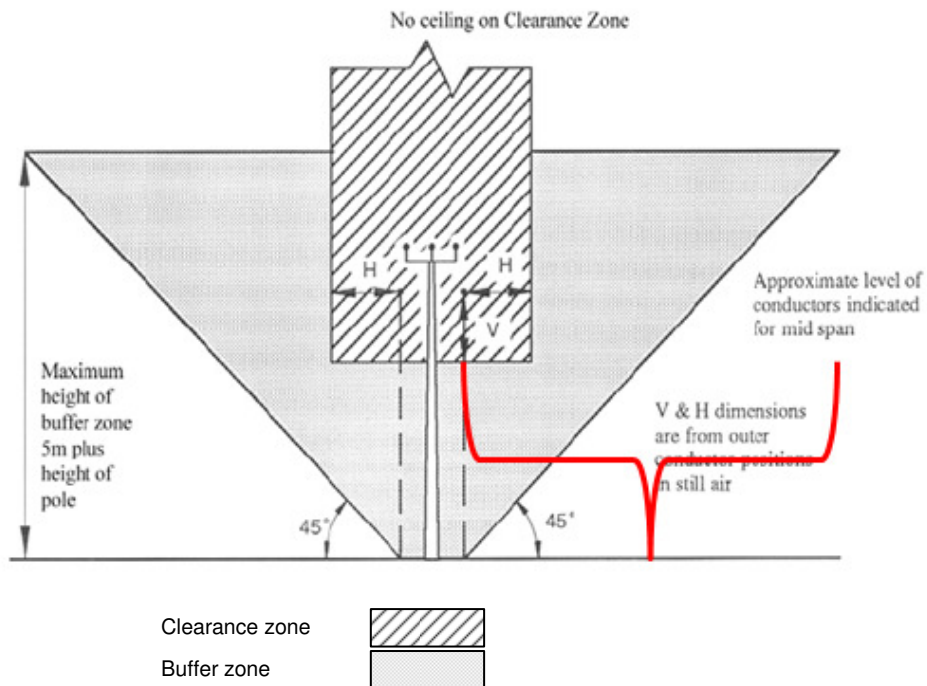
Figure 2-3: Vegetation Clearance Corridor – Bushfire Risk Area 33kV to 66kV
