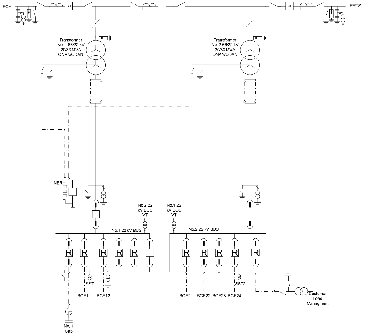
Figure 2: BGE Current Single Line Diagram
