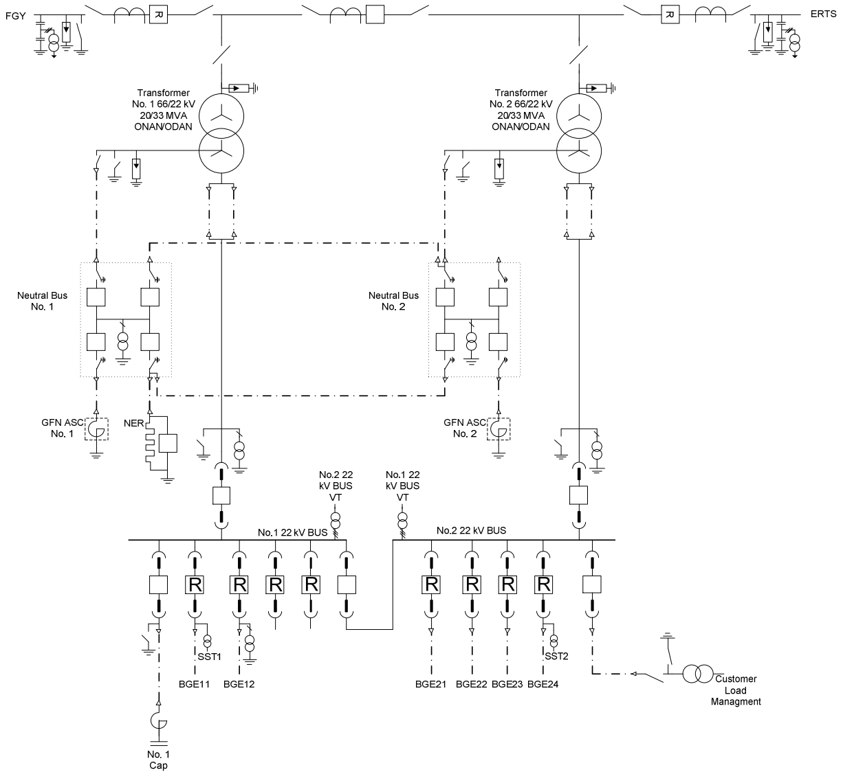
Figure 3: BGE proposed single line diagram
