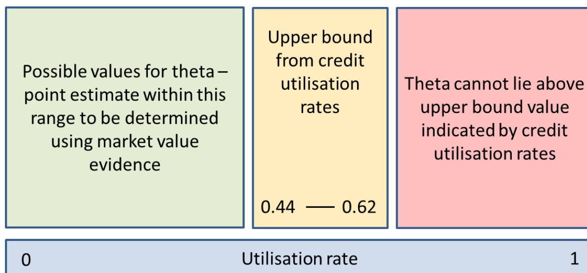
Figure 3: Approach to determining theta
