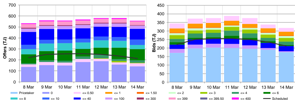
Figure 2.2: SYD daily hub offers and daily hub bids in price bands ($/GJ)
