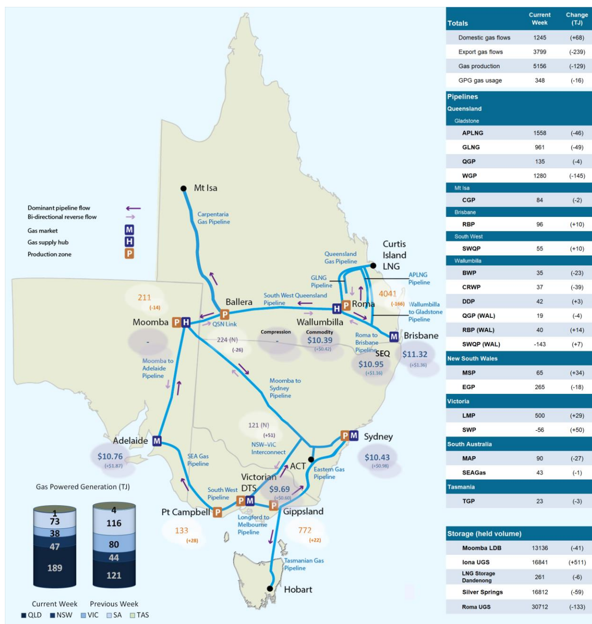
Figure 5.1: Gas market data ($/GJ, TJ/day); Bulletin Board flows (TJ/day) 15
