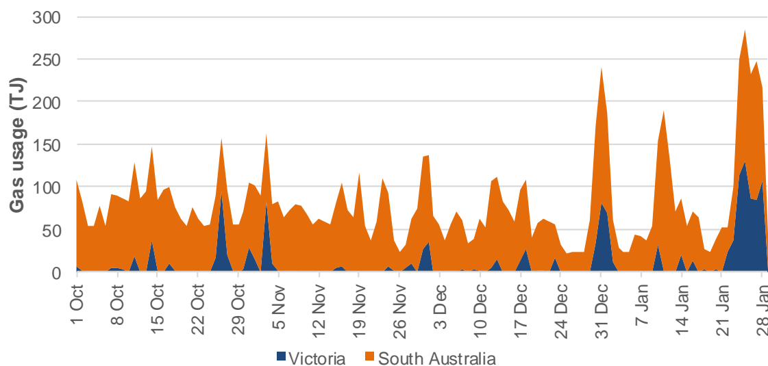
Figure 7: Gas powered generation in Victoria and South Australia (TJ)
