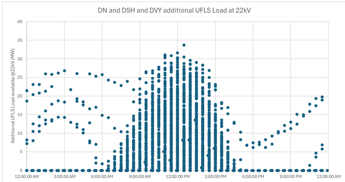
FIGURE 4 DANDENONG, DANDENONG SOUTH, AND DANDENONG VALLEY LOOP ADDITIONAL LOAD @22kV (BY TIME)
