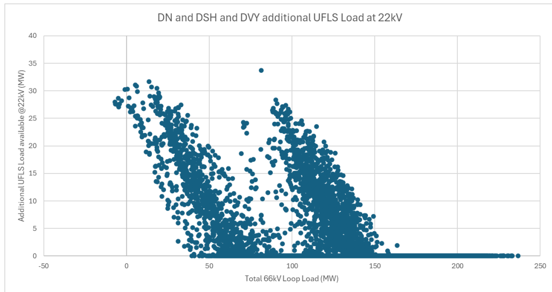
FIGURE 3 DANDENONG, DANDENONG SOUTH, AND DANDENONG VALLEY LOOP ADDITIONAL LOAD @22KV (BY TOTAL LOAD)
