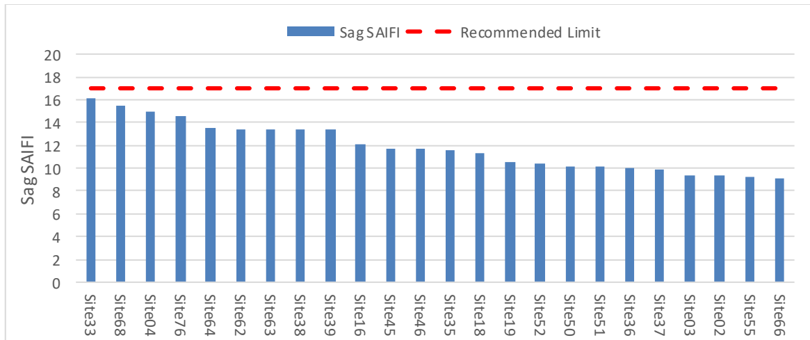
Figure 17.10 Voltage Sag SAIFI for MV sites
