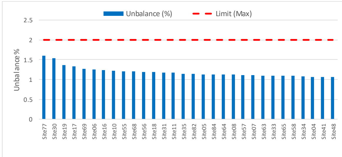
Figure 17.6 Voltage Unbalance at ZSS
