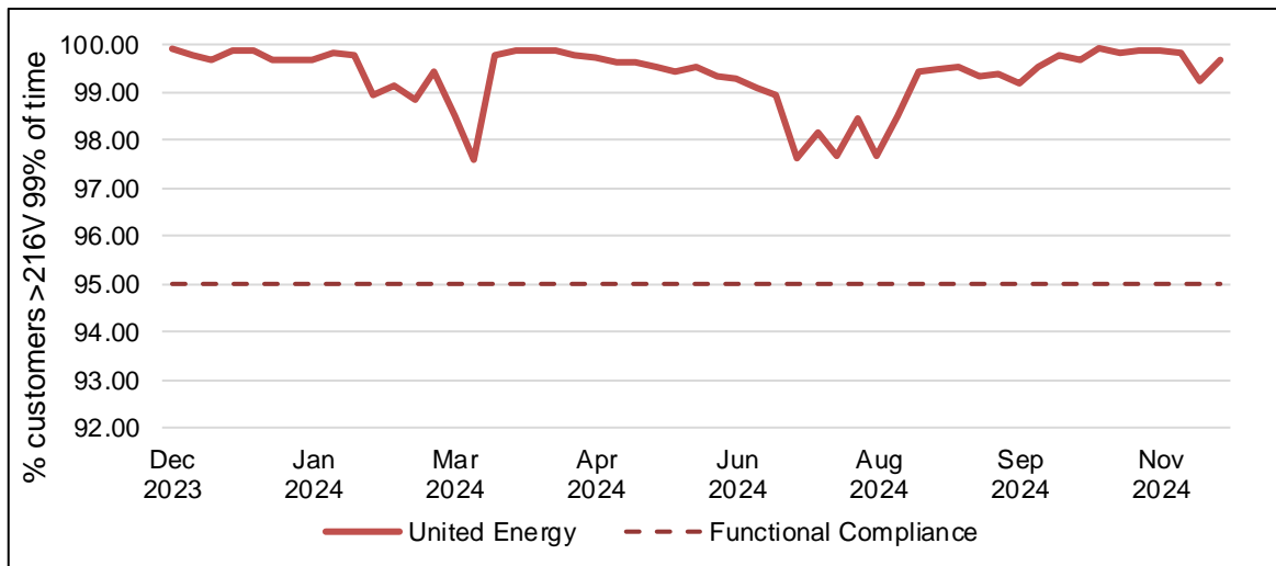
Figure 17.4 Monthly V1% 216V Customer Compliance Dec 2023 – Nov 2024
