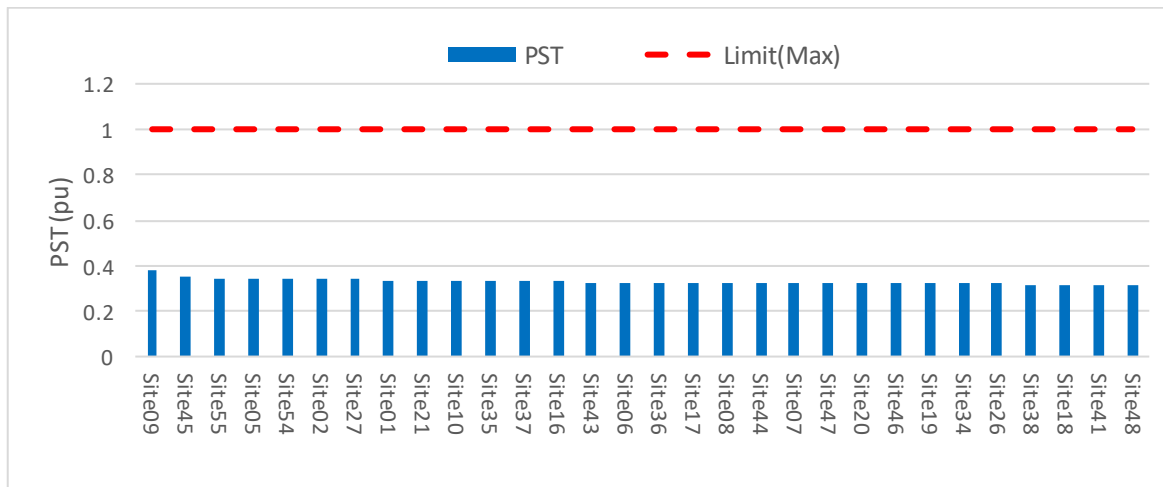
Figure 17.8 Zone Substation Short-term flicker
