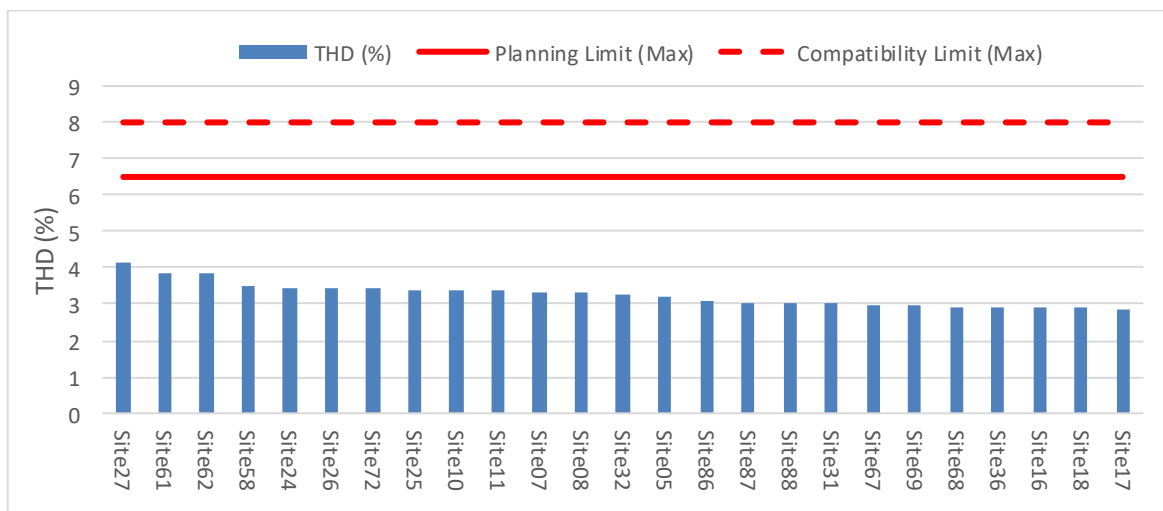
Figure 17.7 Voltage harmonics distribution at Zone Substation Level
