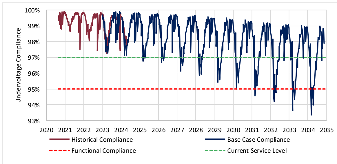
Figure 17.5 Undervoltage compliance historical performance and 2025-2035 forecast
