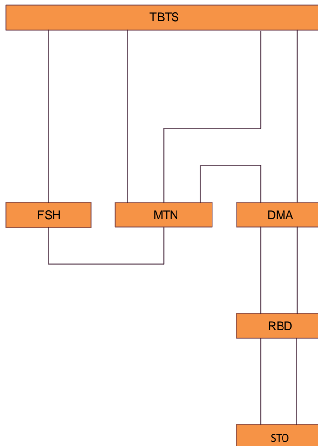
Figure 8.1 TBTS-FSH-MTN-DMA-TBTS sub-transmission system
