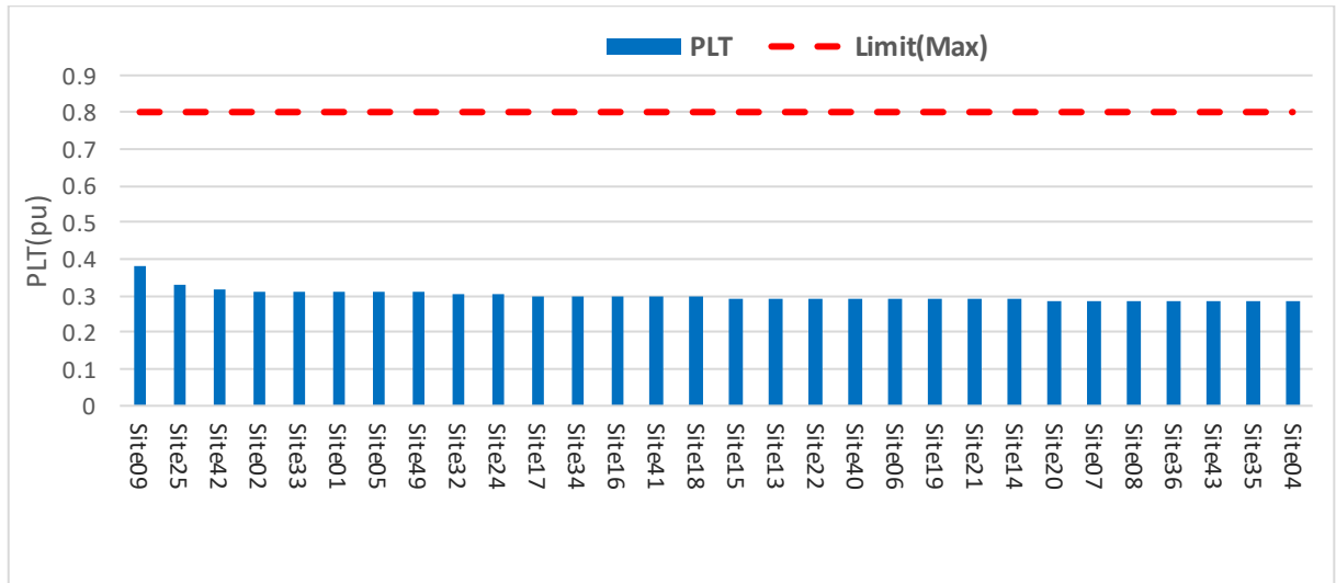
Figure 17.9 Zone Substation Long-term flicker
