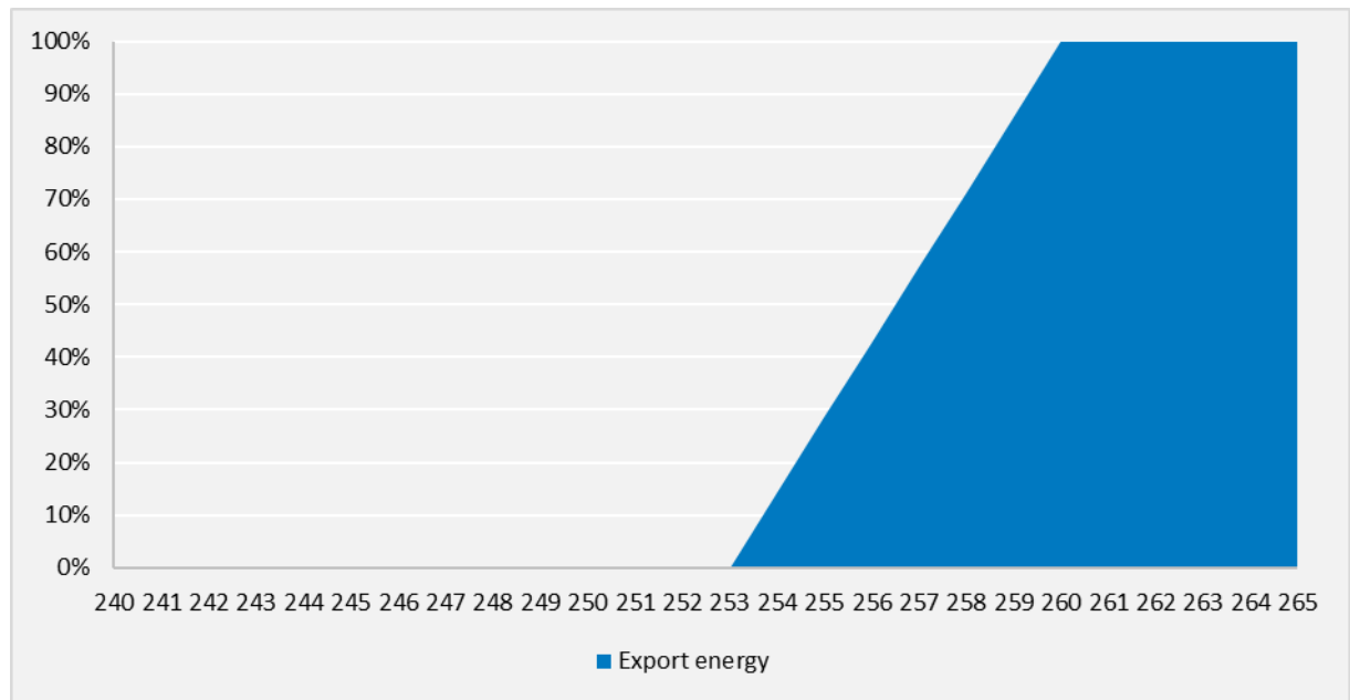
FIGURE 23 SCALING OF ENERGY LOST TO OVERVOLTAGE (V)
