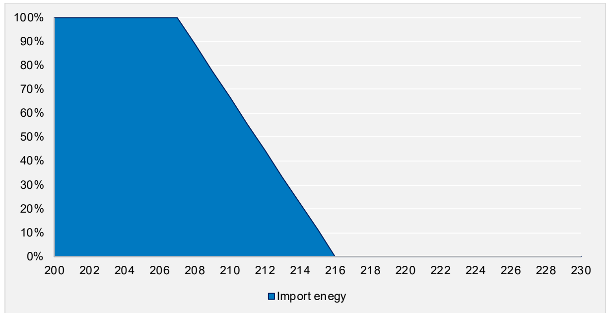
FIGURE 20 SCALING OF ENERGY LOST TO UNDERVOLTAGE (V)
