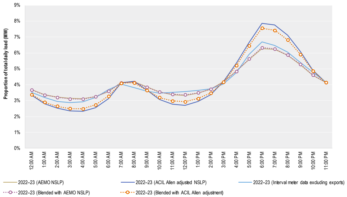
Figure 5.2 Energen load profile inputs
