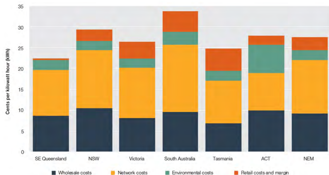
Figure 4: Cost contributions to residential electricity bills averaged across the NEM.
