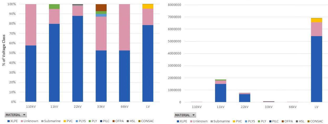
Figure 7: Ergon Energy Breakdown Of Cable Type By Voltage Class
