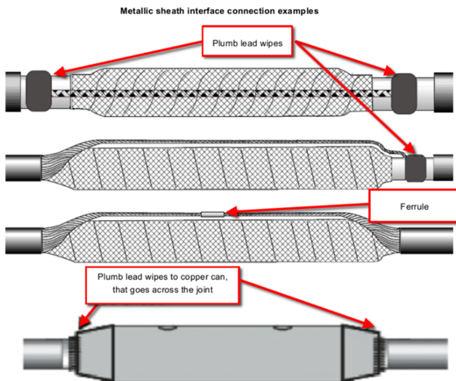
Figure 17: Metallic sheath bonding and mechanical ferrule connection
