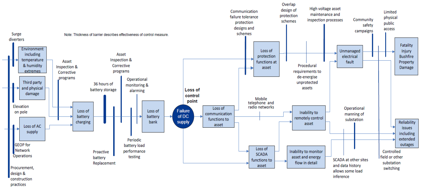
Figure 15: Lines asset DC supply threat barrier diagram
