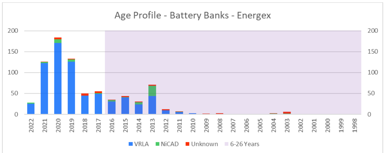
Figure 5: Energex Region substation battery bank age profile
