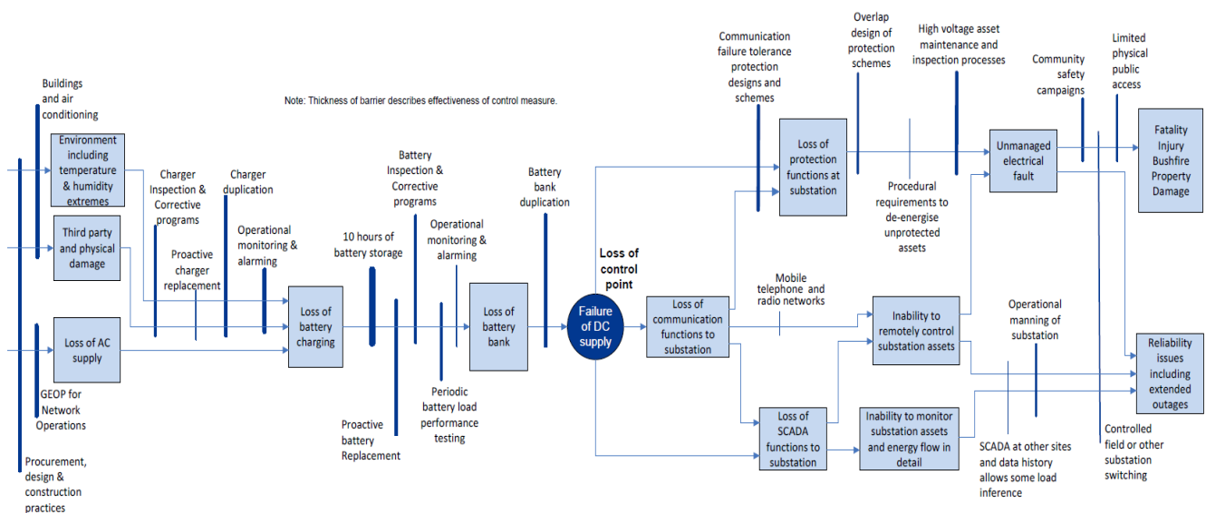
Figure 14: Substation DC system threat barrier diagram
