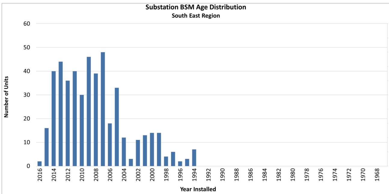
Figure 7: Energex Region substation battery system monitor (BSM) age profile
