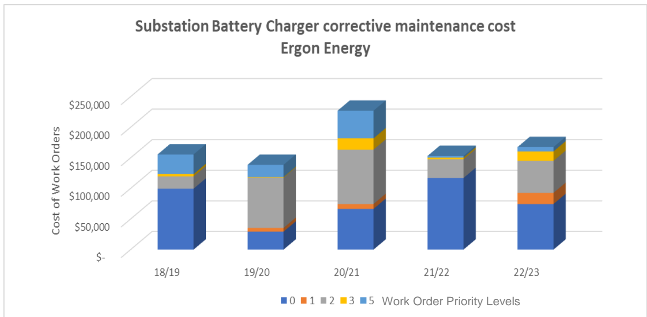
Figure 9: Substation battery charger corrective work orders – Ergon Energy Region
