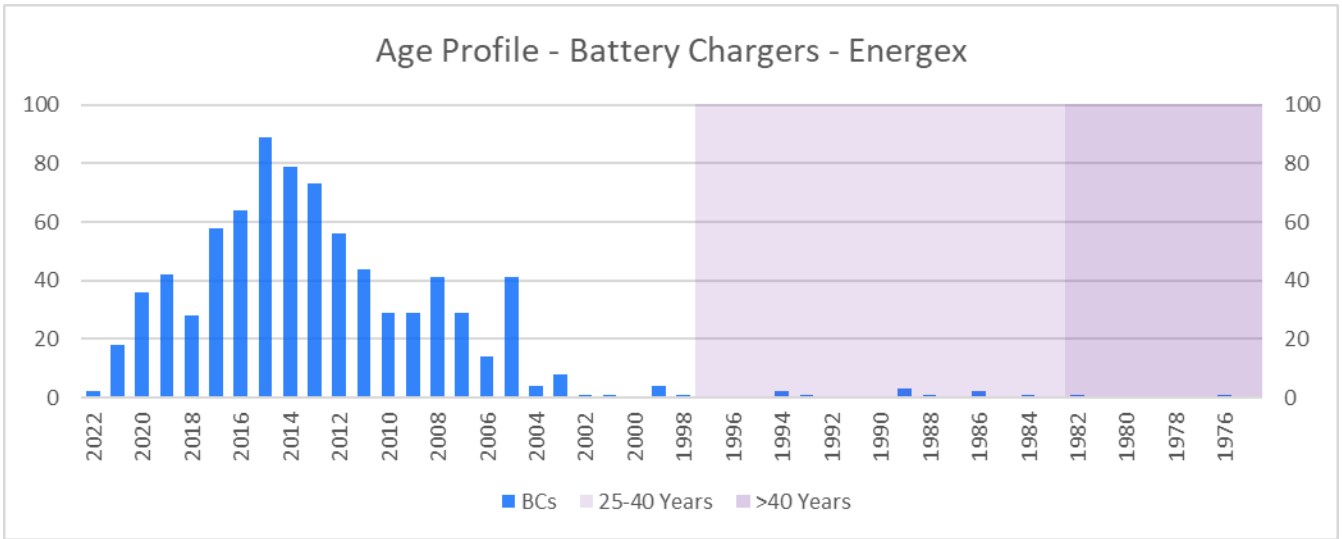
Figure 6: Energex Region substation battery charger age profile
