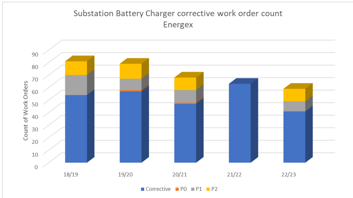
Figure 12: Energex region substation battery charger corrective maintenance
