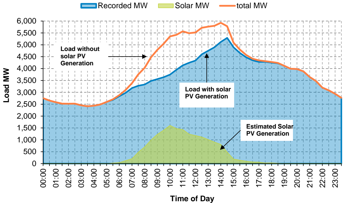
Figure 6 – System Demand – Solar PV Impact, 2 February 2022
