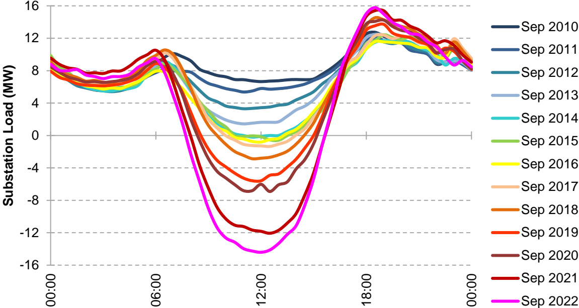
Figure 28 – Spring Load Profile with increasing Solar PV of North Maclean Zone Substation
