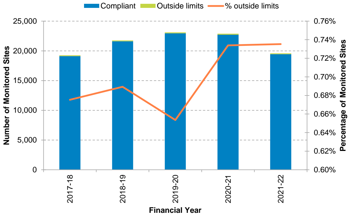
Figure 24 – Number of Monitored Sites Reporting Under Voltage
