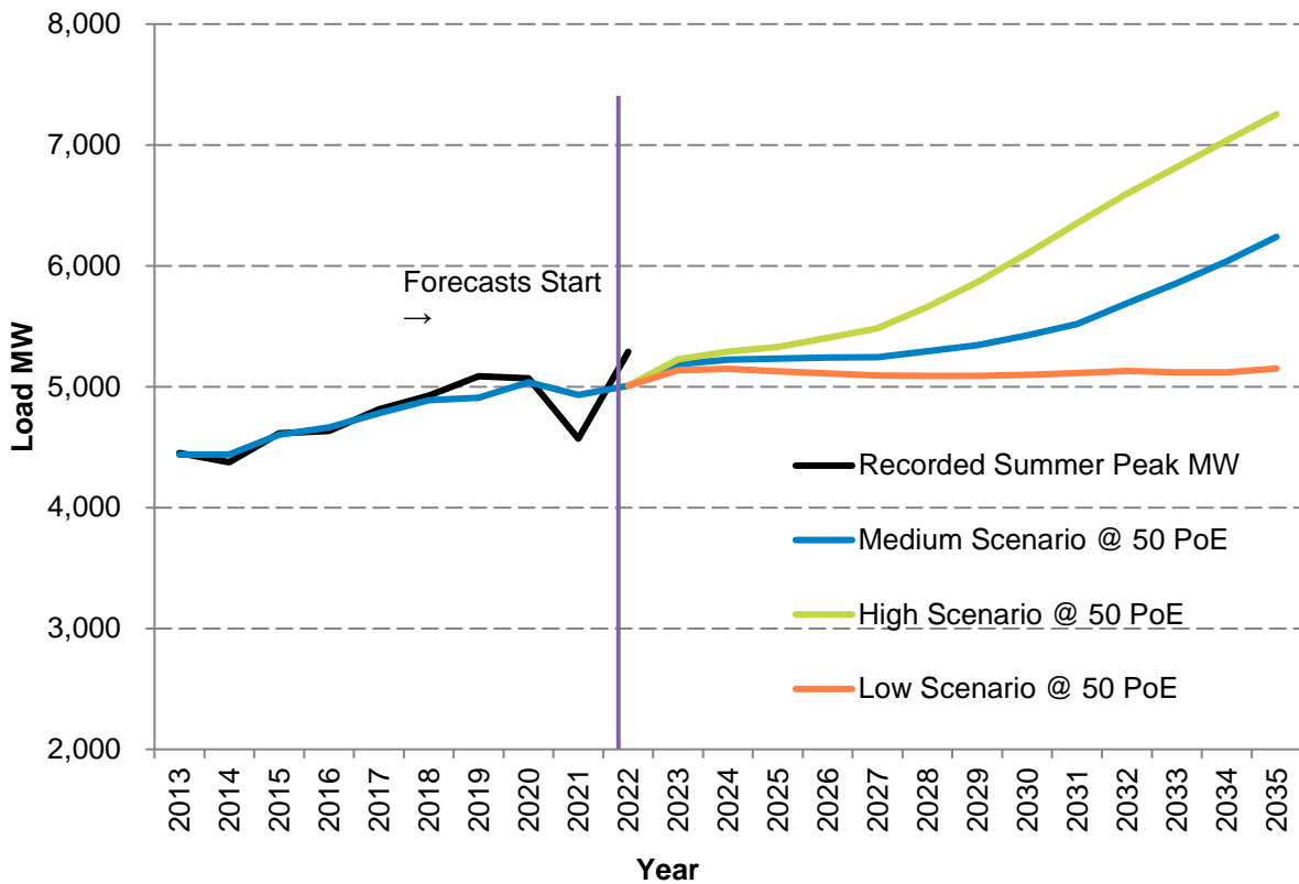
Figure 7 – Three Scenarios of EGX Summer Peak MW Forecasts @ 50 PoE Level
