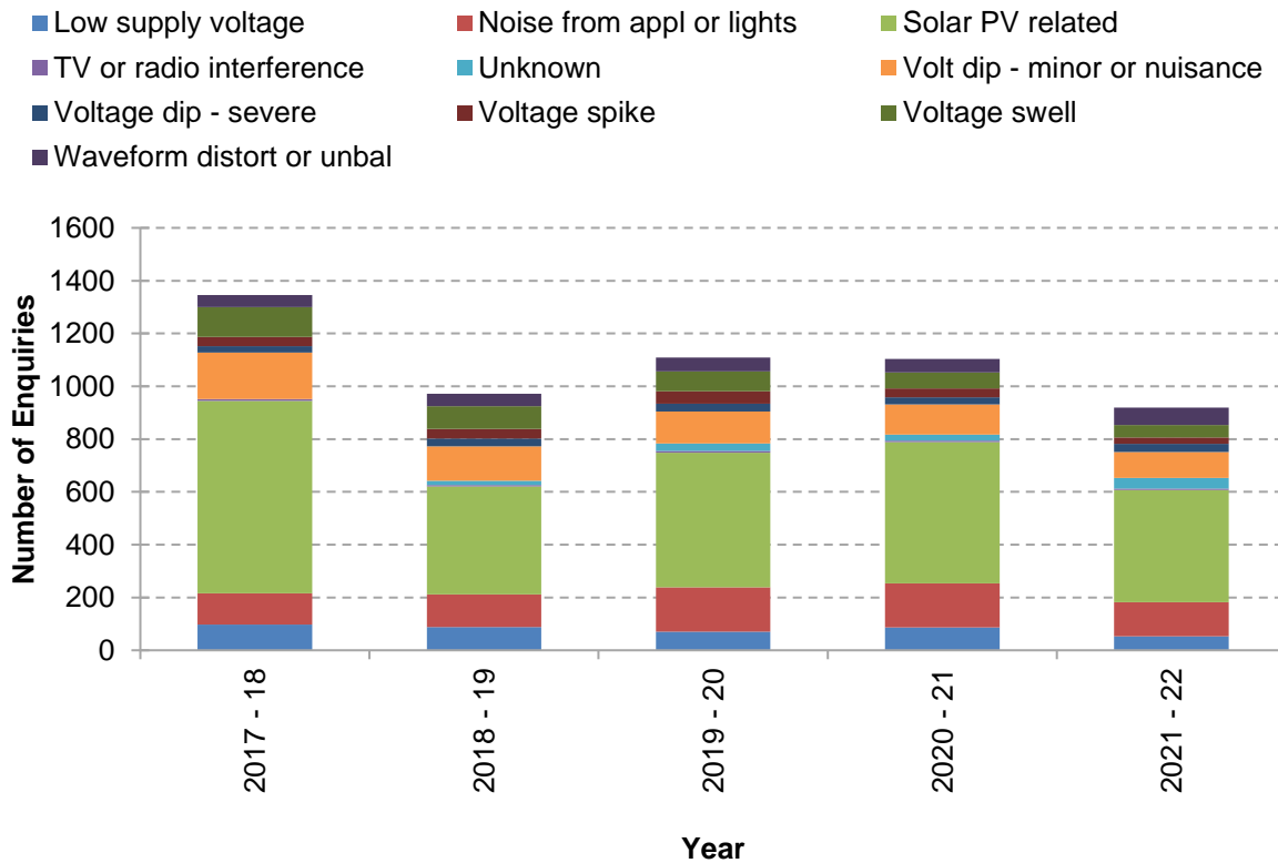
Figure 21 – Quality of Supply Enquiries per Year
