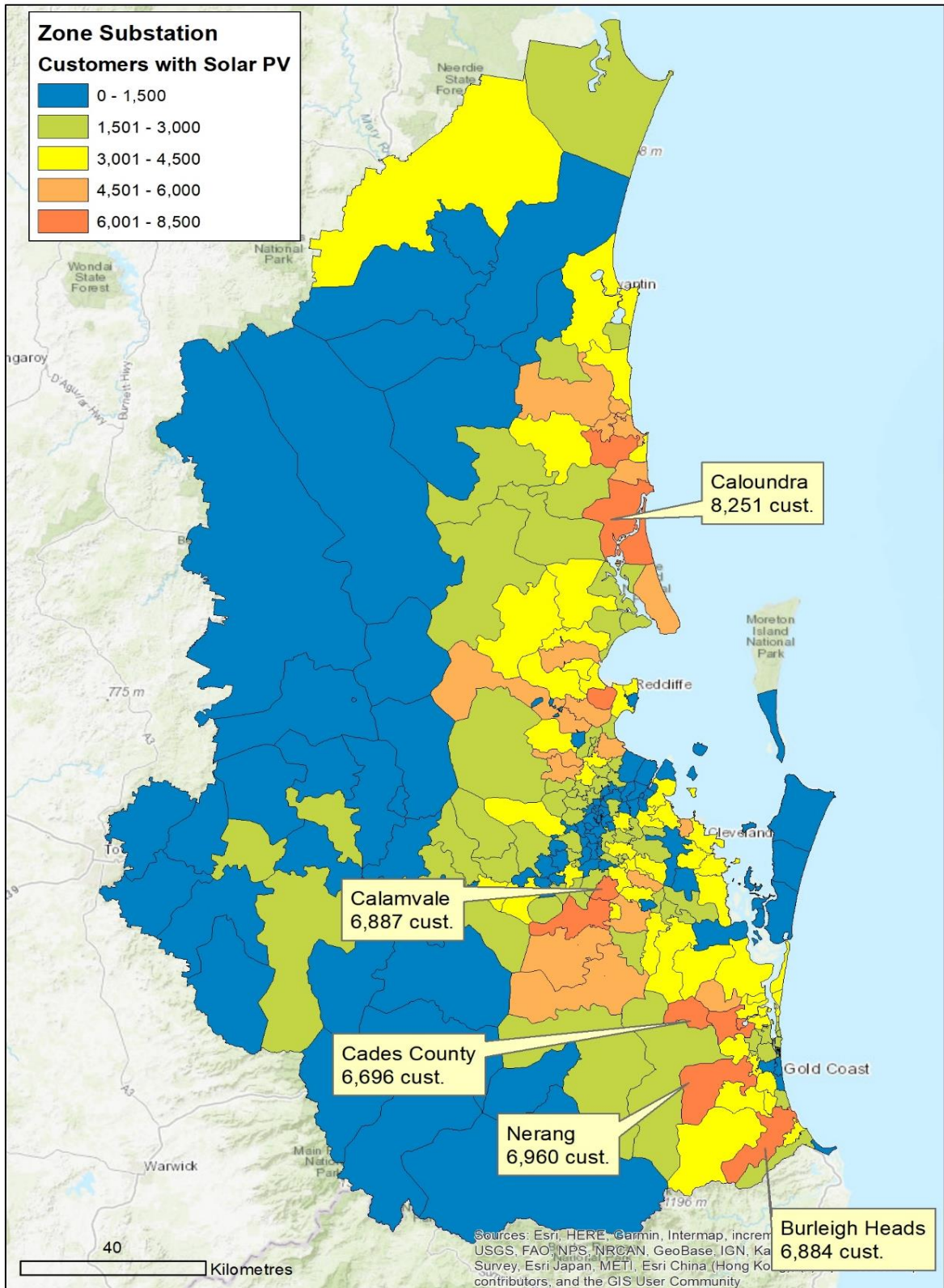
Figure 29 – Number of customers with Solar PV by Zone Substation
