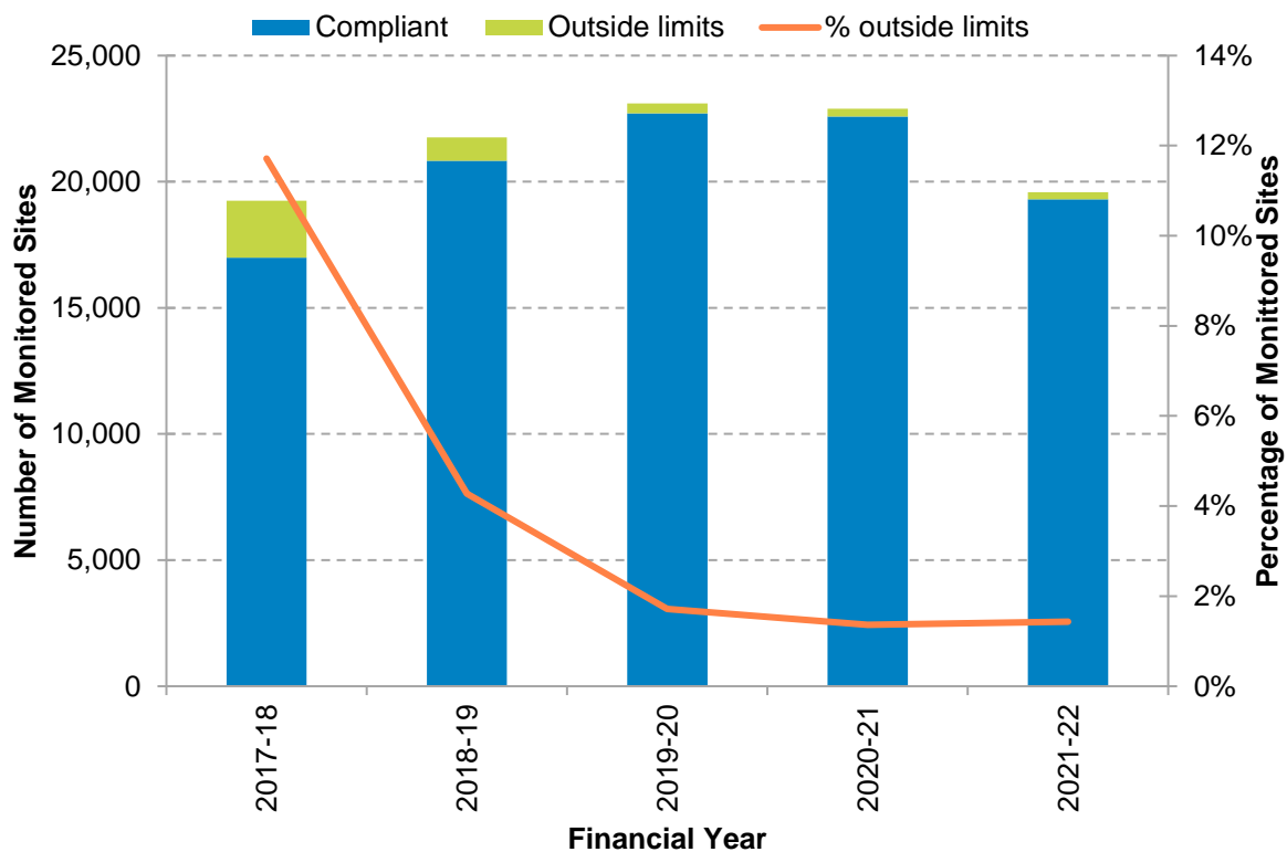
Figure 23 – Number of Monitored Sites Reporting Overvoltage
