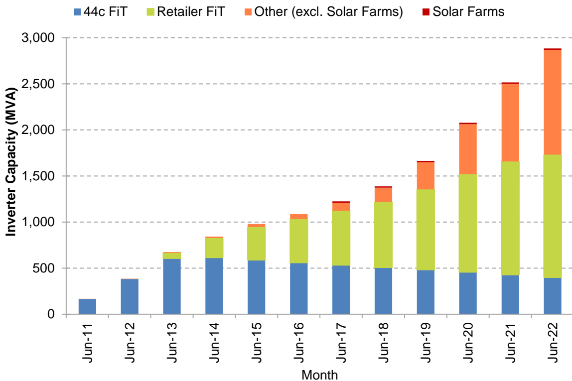
Figure 27 – Grid Connected solar PV System Capacity by Tariff as at June 2022
