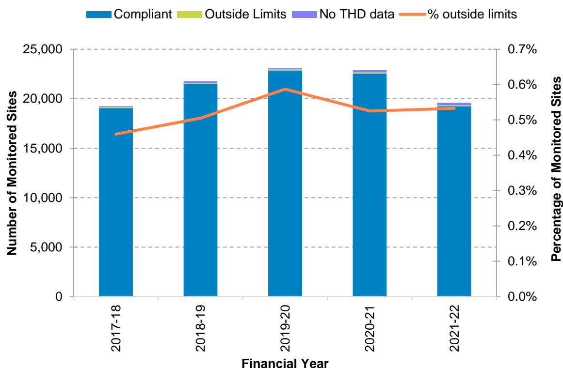
Figure 26 – Number of Monitored Sites Reporting Total Harmonic Distortion
