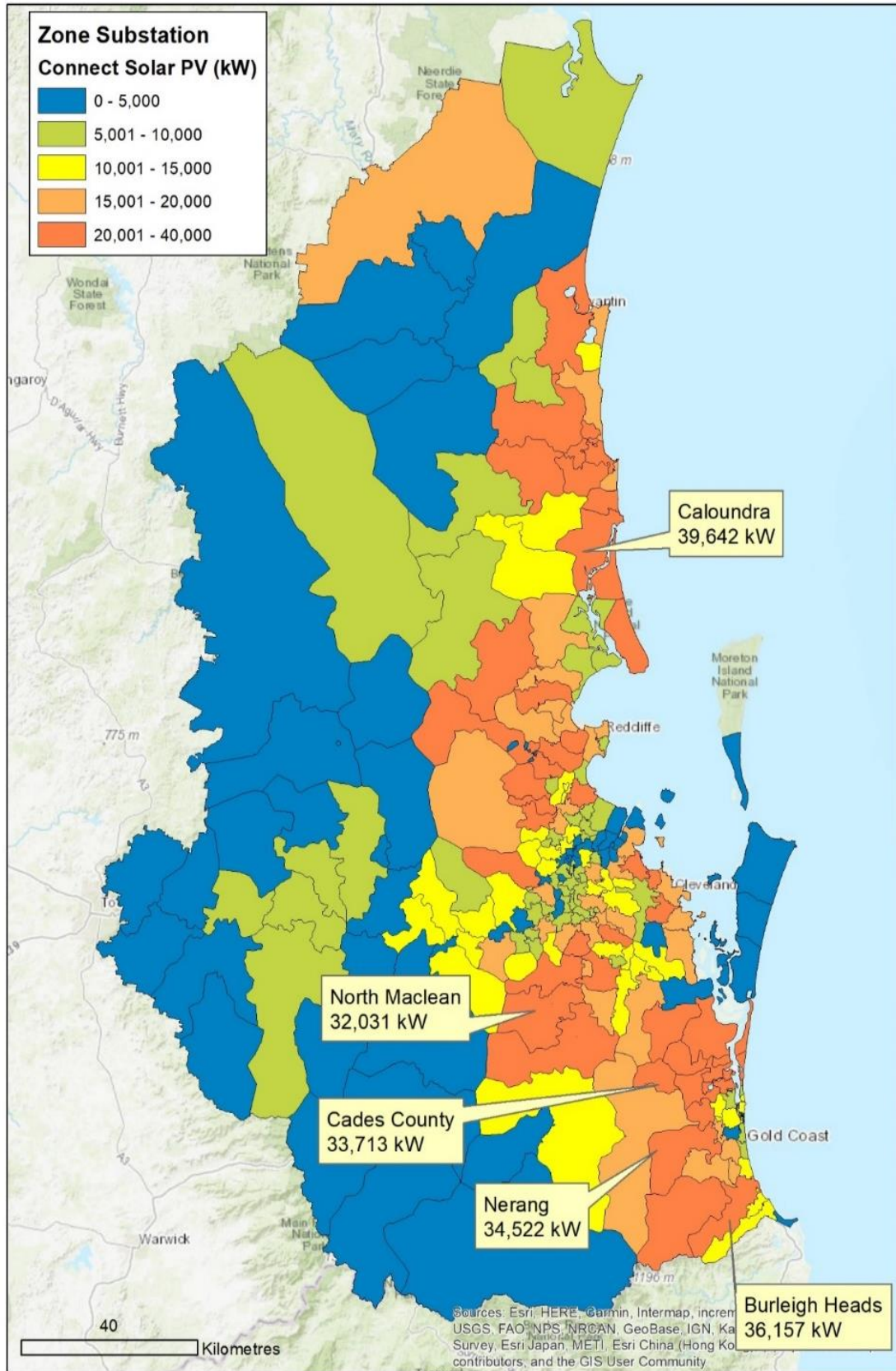
Figure 30 – Installed Capacity of Solar PV by Zone Substation
