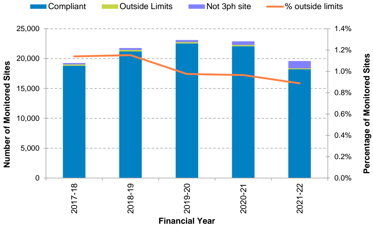
Figure 25 – Number of Monitored Sites Reporting Voltage Unbalance
