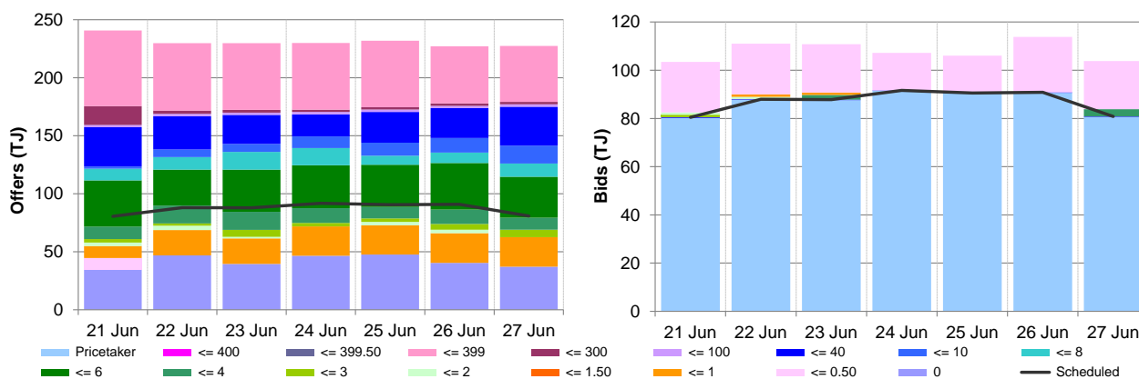
Figure 3.3: ADL net scheduled and allocated gas hub supply (excluding MOS)
