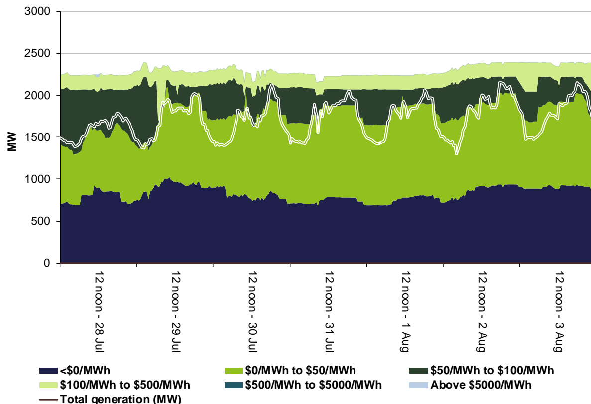
Figure 6: Tasmania generation and bidding patterns
