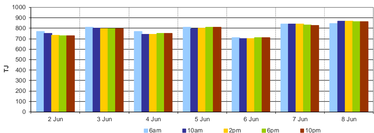
Figure 1.2: Demand forecasts
