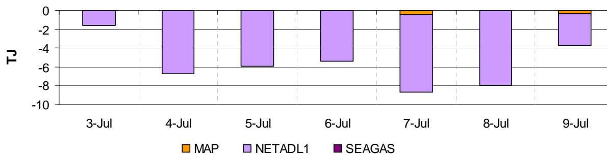
Figure S20: Net Deviations – Adelaide Hub
