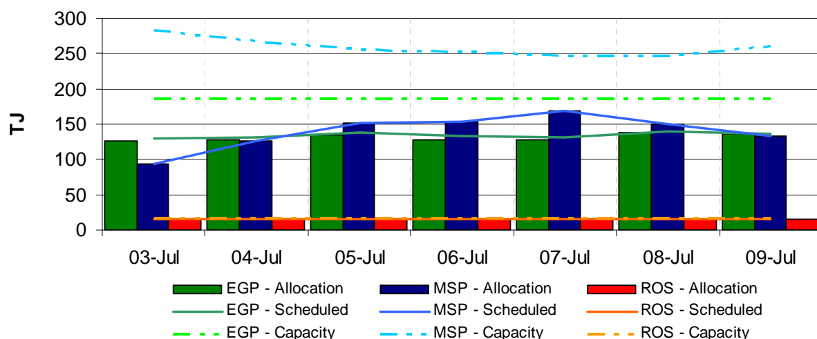
Figure S7: Allocated vs scheduled pipeline quantities - Sydney Hub (TJ)
