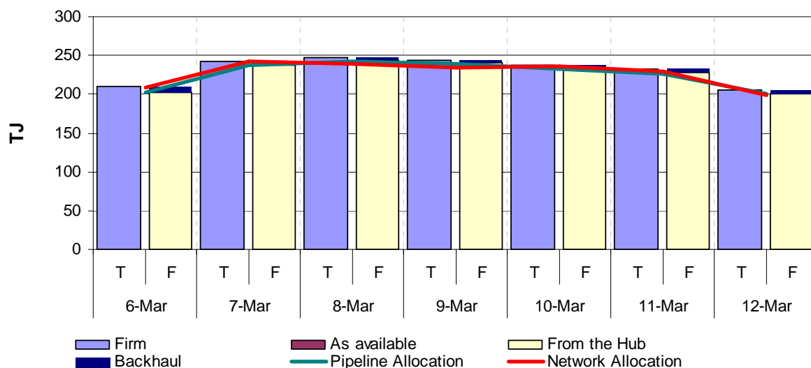
Figure S5: Allocated vs scheduled ex ante quantity - Sydney Hub (TJ)^
